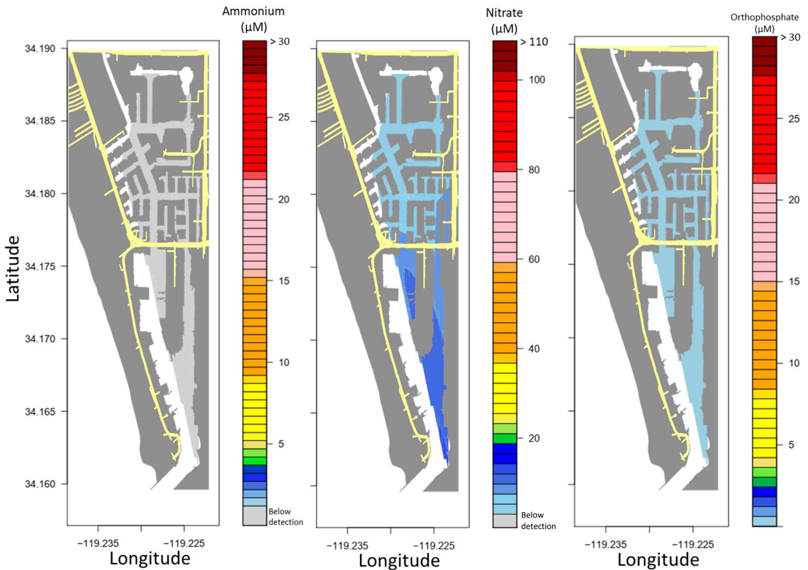
Figure 6. Color contour plots of concentrations of ammonium, nitrate, and orthophosphate in water samples collected in CIH on July 6, 2018. Nitrate was the dominant form of inorganic (nutrient) nitrogen in CIH on the sampling date. Both nitrate and orthophosphate (i.e. nutrient phosphorus) were measurable but not excessively high at the time of sampling (see Figs. 10, 11 for comparison, and Table 1 caption for discussion and interpretation). Data for Seabridge Marketplace plaza was not collected because the boat couldn't access it during the sampling event.
