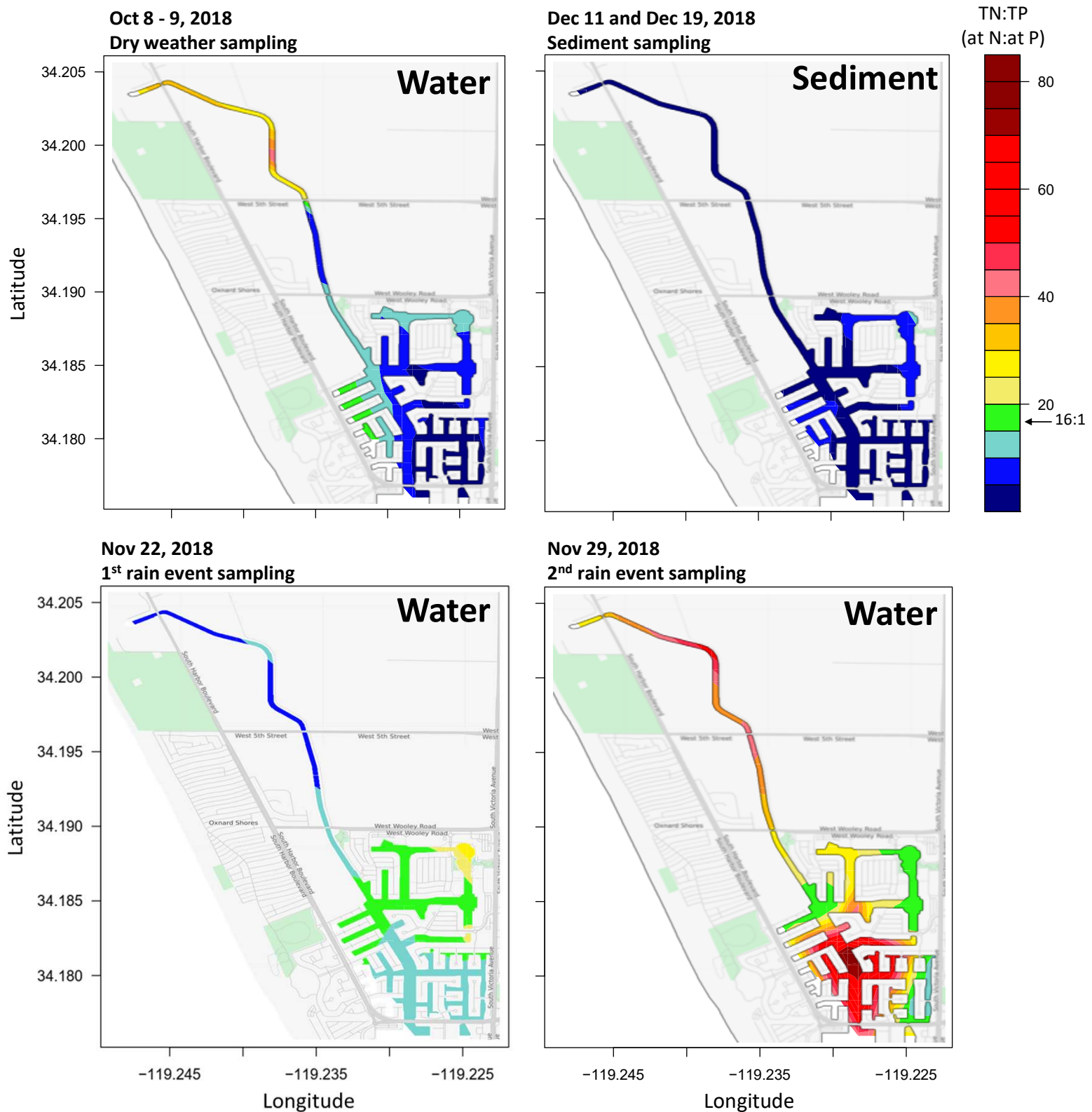
Figure 14. Color contour plots of total nitrogen: phosphorus ratios (TN:TP) in the water column during dry weather sampling (top, left), and following two rain events (bottom left and right), and in the sediments (top, right). The Redfield ratio (16:1) is indicated on the color scale. Total N:P ratios in the water were highly variable among the three sampling dates. Values following rain events tended to be much higher than values during the dry weather sampling. TN:TP ratios in sediments were consistently low across CIH and Edison Canal (top right), indicating loss of nitrogen from the sediments or effective retention of phosphorus (or both) in the sediments of this coastal ecosystem.
